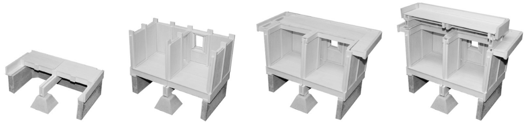
10. Panel-post construction system: 1/2-in. scale model reconstruction of components with their step-by-step assembly. (Model is constructed by Jacob Kwon.)
