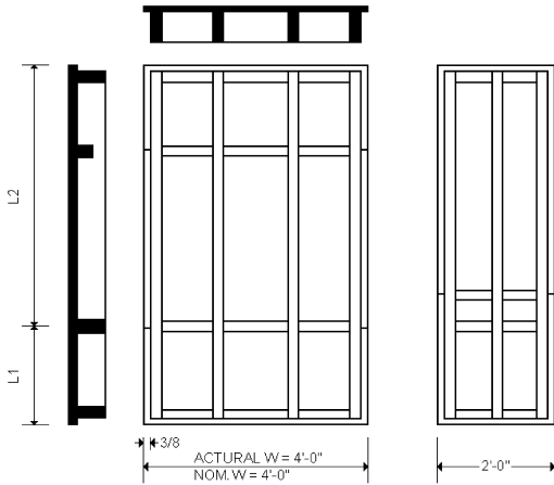
FLOOR PANEL: #FL (W X L1 + L2 & FINISH)
