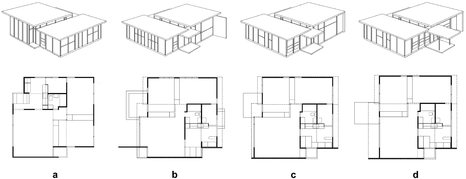
3. Rudolph M. Schindler, panel-post construction. Four variations of a standard two-bedroom unit with their axonometric. (Drawings are redrawn by the author.)
