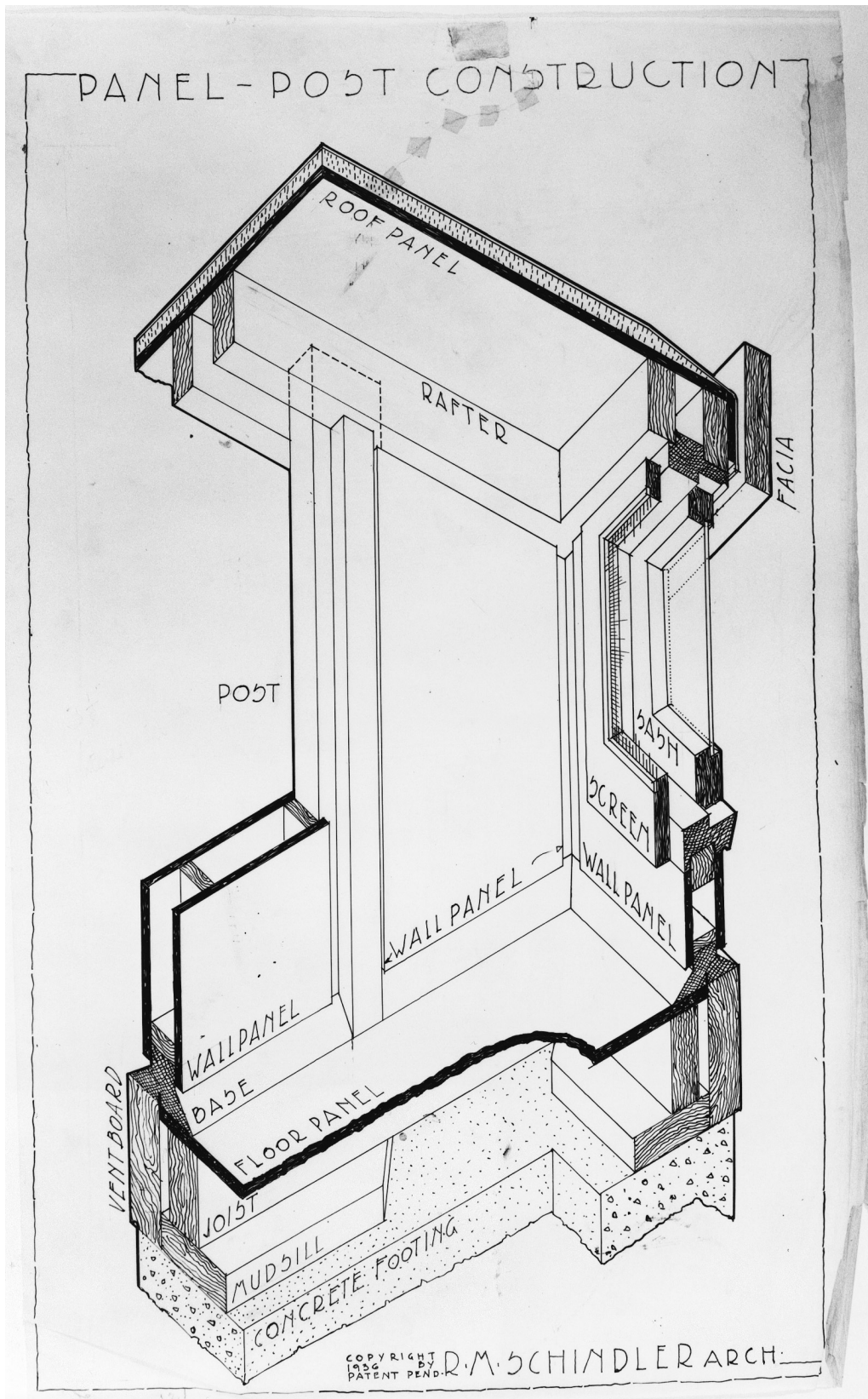
9. Cross section of a typical panel-and-post connection. (R.M. Schindler Collection, Architecture and Design Collection, University of California, Santa Barbara, CA.)
