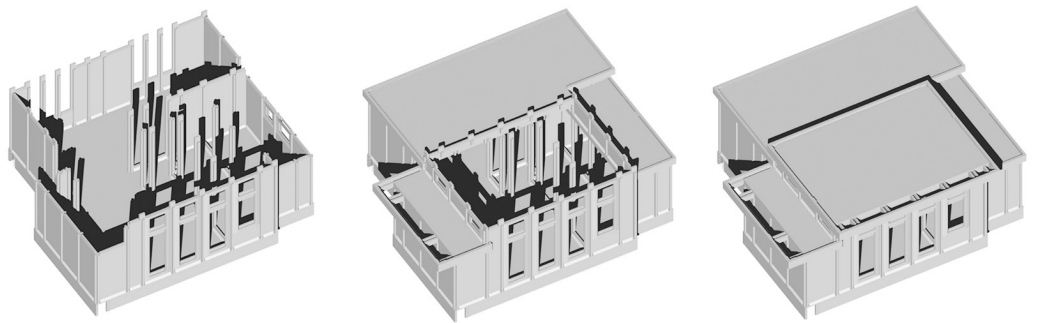
11. Computer generated unit model with the panel-post construction system.
