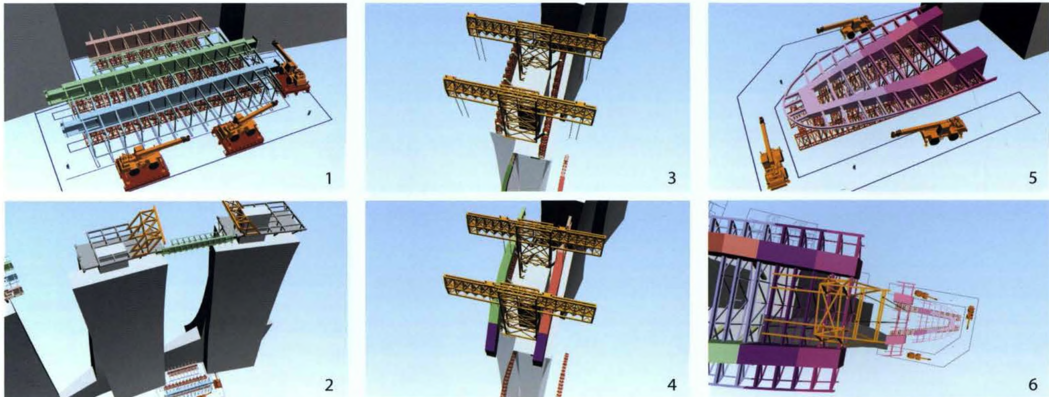
Figure 11. Diagrammatic phasing of erecting the SkyPark
